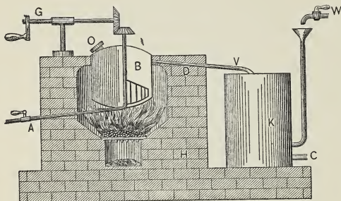
FIG. 15.—Andrès' Gum-melting Furnace.
